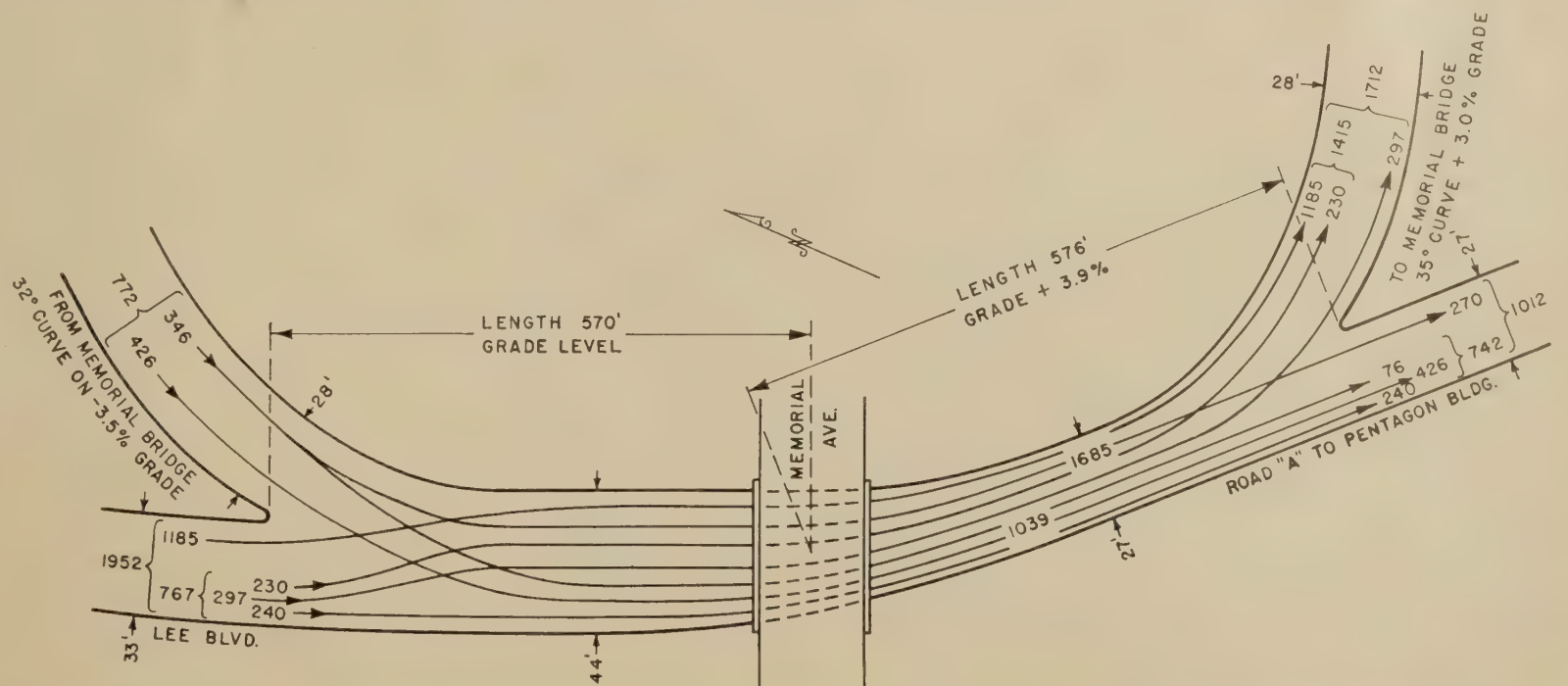
Figure 40.—Maximum observed hourly traffic volume on mixing lane section on roadway under Memorial Avenue near west end of Memorial Bridge, Washington, D. C.
